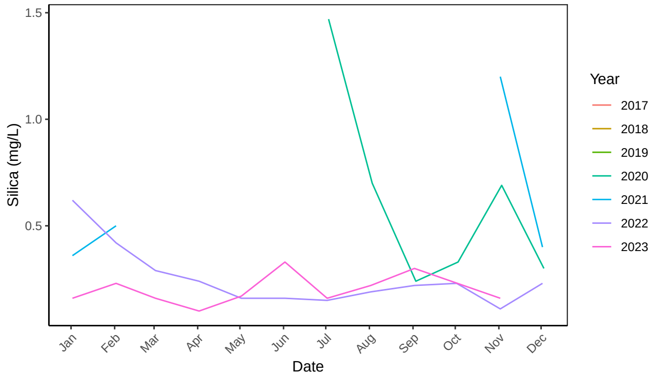
B2 Raceway 1 Silica (mg/L) Monthly Median
